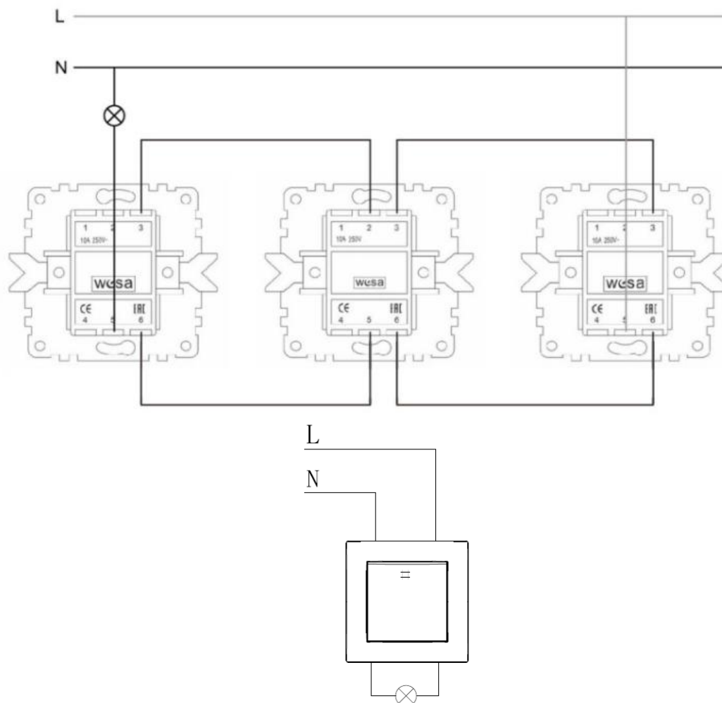
WESA 01-A cross switch - connection diagram with stair switch
